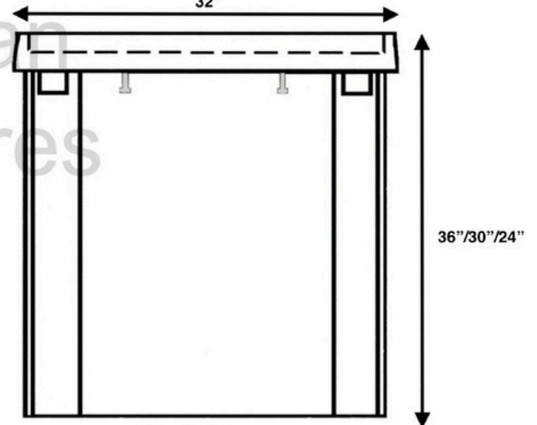
End View
